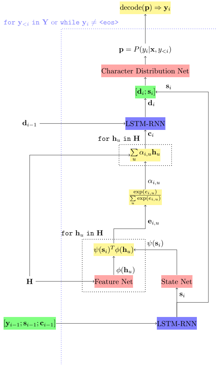
Figure 5.15: A different attend and spell cell configuration, featuring an additional post context RNN
