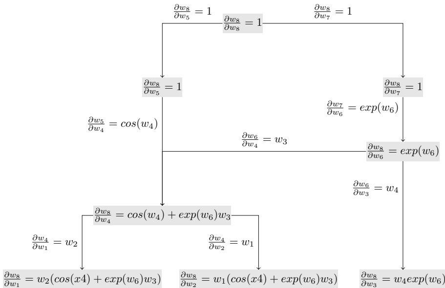
Figure 2.5: Reverse sweep.
