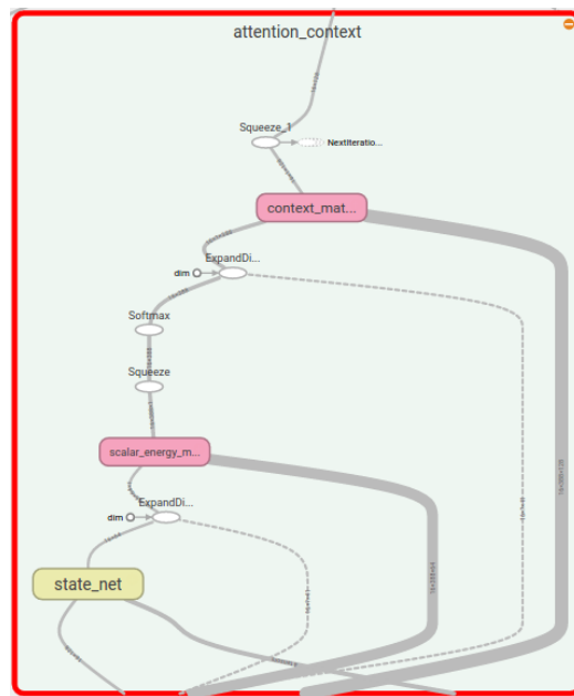
Figure 4.2: Tensorboard visualization of the attention context computations.
