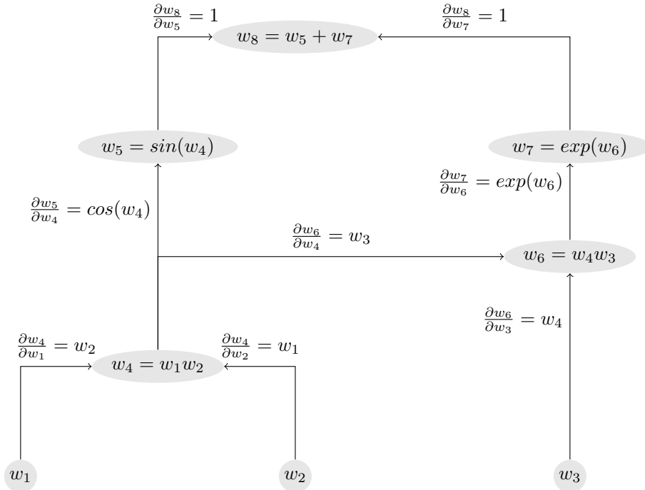
Figure 2.4: Example function network with partial derivatives.
