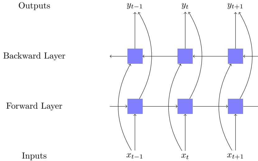
Figure 2.10: A bidirectional Long short term memory layer, according to [16]
