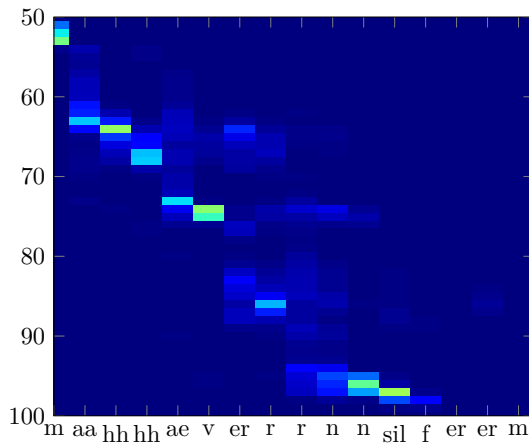
Figure 5.7: Closeup on interesting parts of the first third of the attention matrix.
