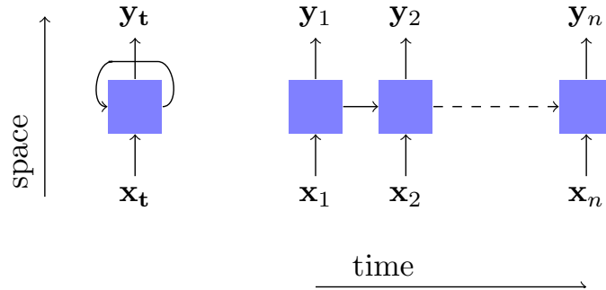
Figure 2.8: Rolled (left) and unrolled (right) recurrent neural net with two units.
