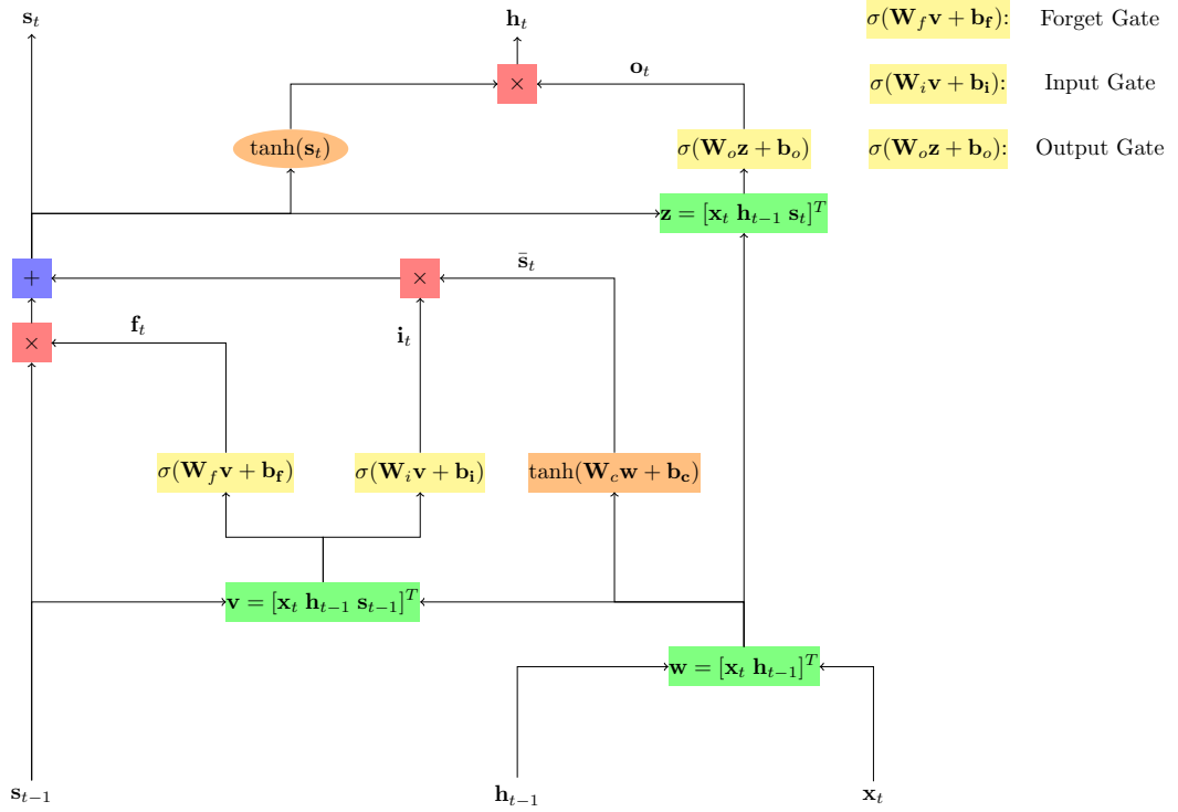
Figure 2.9: Visualization of the LSTM architecture.
