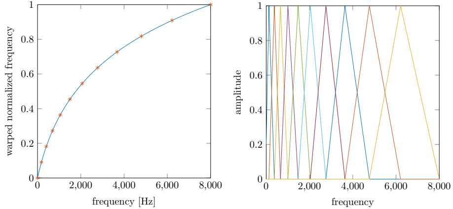
Figure 2.2: The Mel-scale (blue) with Mel-Frequency Cepstrum Coefficients (red) is shown on the left. Filterbanks with Mel-spaced filters are depicted on the right.
