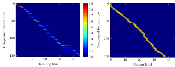
Fig. 2. Plot of the alignment vectors computed by the network for all 45 labels assigned to timit utterance fm1d0_sx295 (left), and alignments assigned by a human listener (right).
