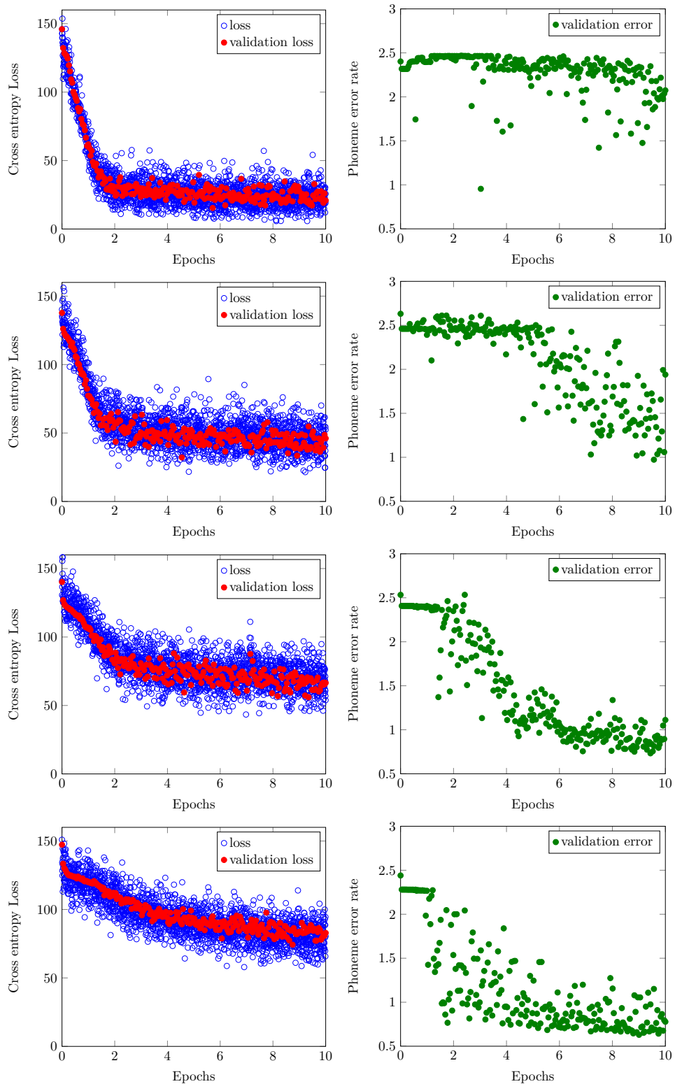
Figure 5.11: Repetitions of the same experiment with increasing network output reuse probabilities 0.2, 0.4, 0.6, 0.8, one experiment per row.
