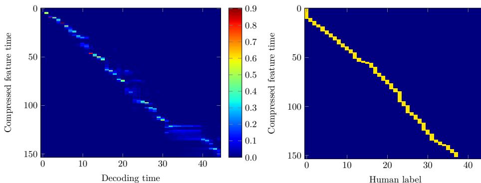
Figure 5.6: Plot of the alignment vectors computed by the network for all 45 labels assigned to timit utterance fm1d0_sx295 (left), and alignments assigned by a human listener (right).
