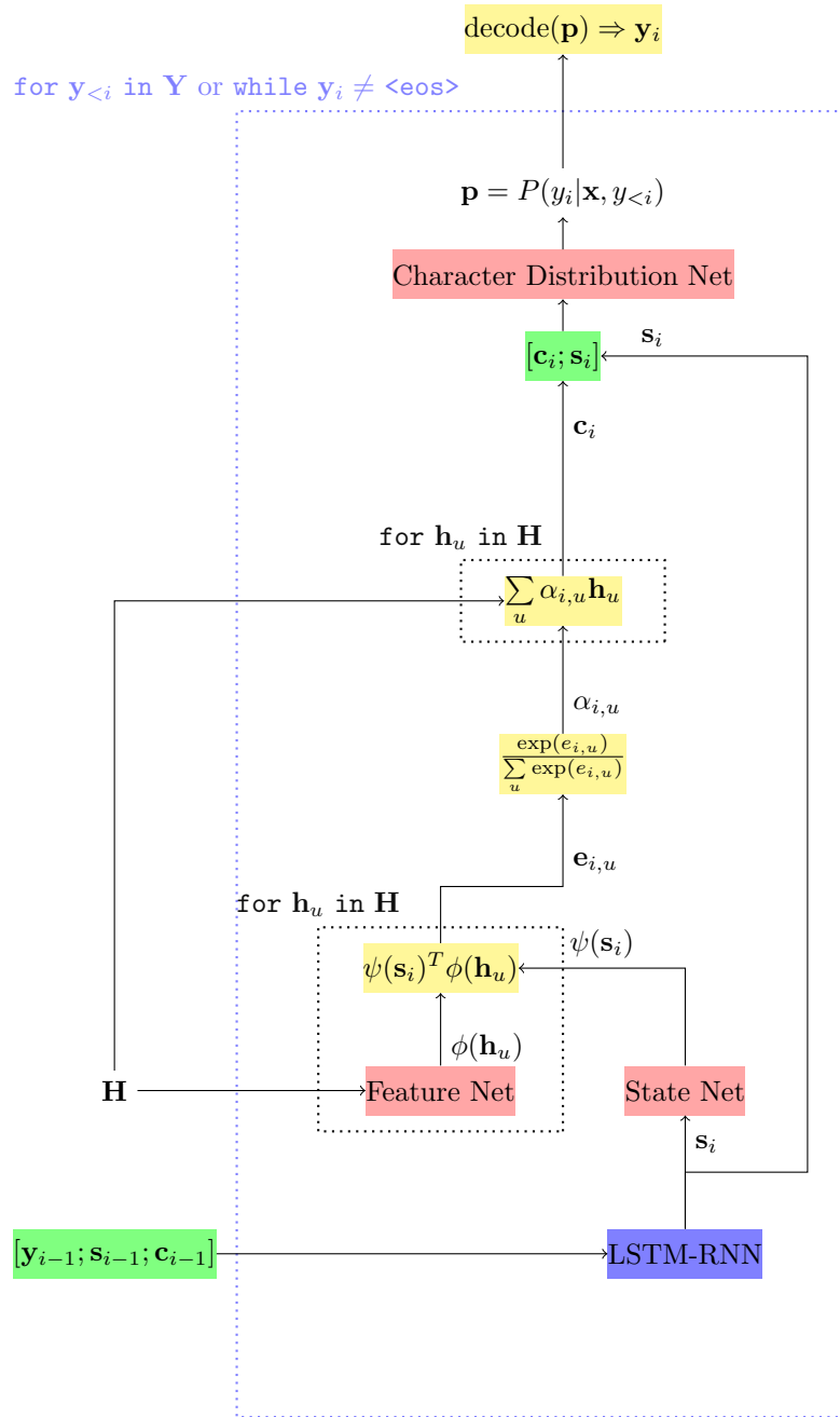
Figure 4.1: Schematic of the attend and spell cell components.
