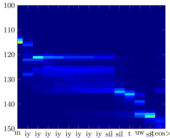
Figure 5.8: Closeup on interesting parts of the second third of the attention matrix.
