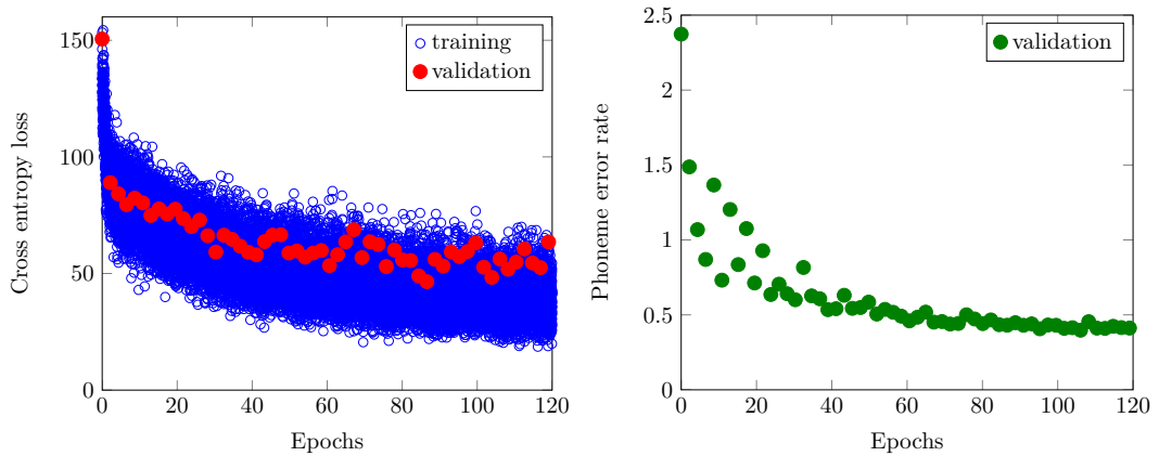
Figure 5.14: Dropout LAS learning curves with a listener LSTM using 128 units per direction and one PLSTM. The speller LSTM state size was set to 256. All feed-forward networks in the speller had 128 units per layer and two layers overall.
