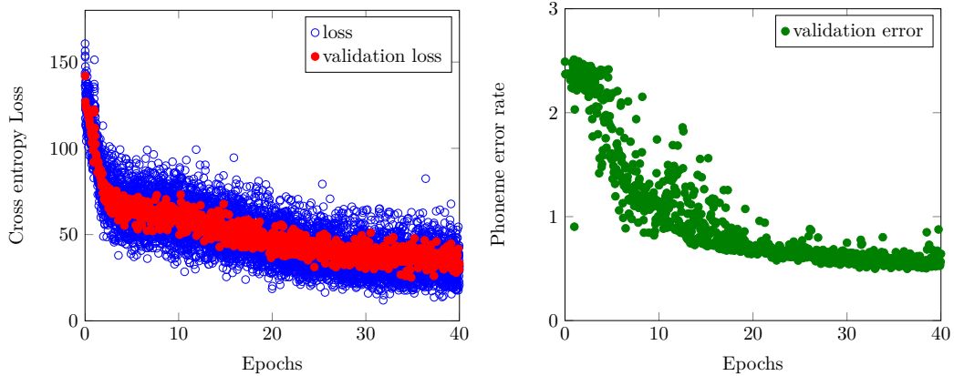
Figure 5.12: Training full las over 40 epochs with a network output reuse probability of 0.5.
