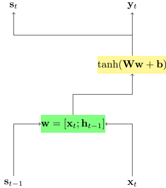
Figure 2.7: Visualization of a single recurrent cell.
