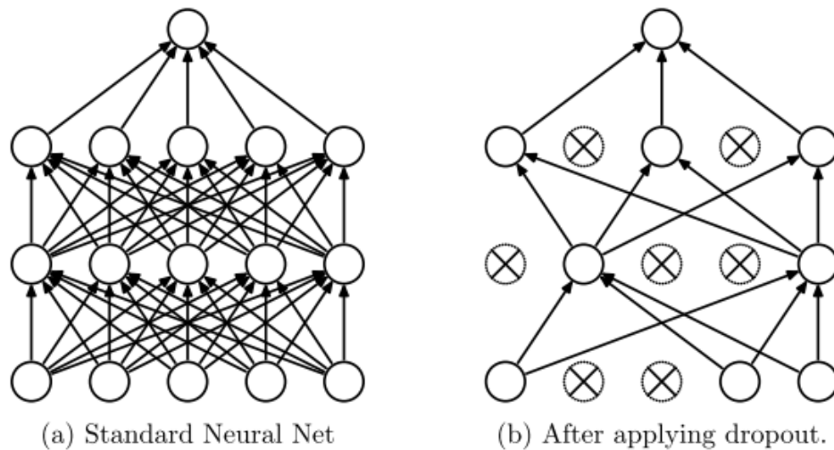
Figure 2.6: “Dropout Neural Net Model. Left: A standard neural net with 2 hidden layers. Right: An example of a thinned net produced by applying dropout to the network on the left. Crossed units have been dropped.” [27], image and caption taken from the same source.
