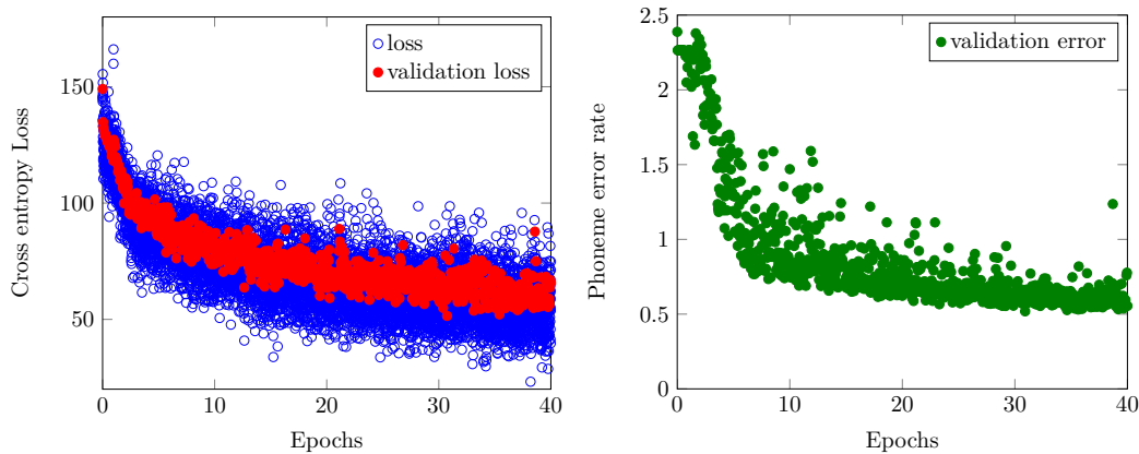
Figure 5.5: The training progress shown for the full las architecture with greedy decoding, over 40 epochs, network output reuse probability 0.7 and input noise standard deviation 0.65 .
