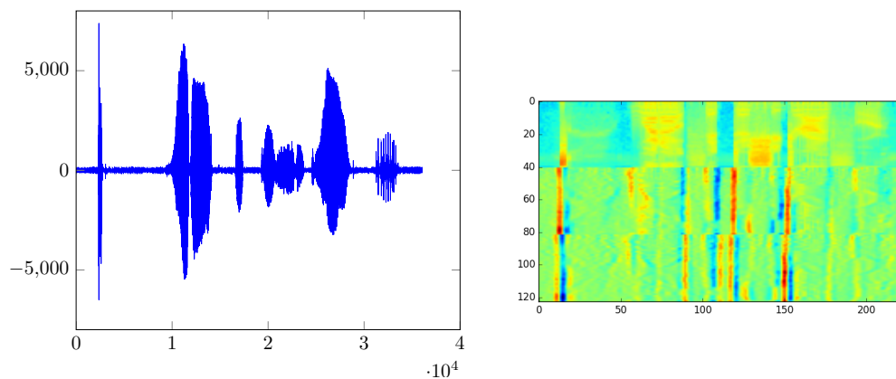
Figure 5.2: Raw time domain signal and feature vectors. Features include 40 mel banks as well as the first and second derivatives. Raw data was taken from TIMIT utterance faem0-si2022 “What outfit does she drive for?”.
