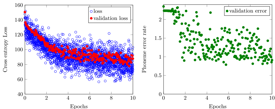
Figure 5.10: Learning curves of the las architecture with an additional post context LSTM block. Greedy decoding was used as well as training network output reuse probability of 0.7.
