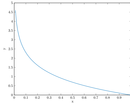
Figure 2.3: Plot of y = -\ln(x) for x \in (0, 1) .
