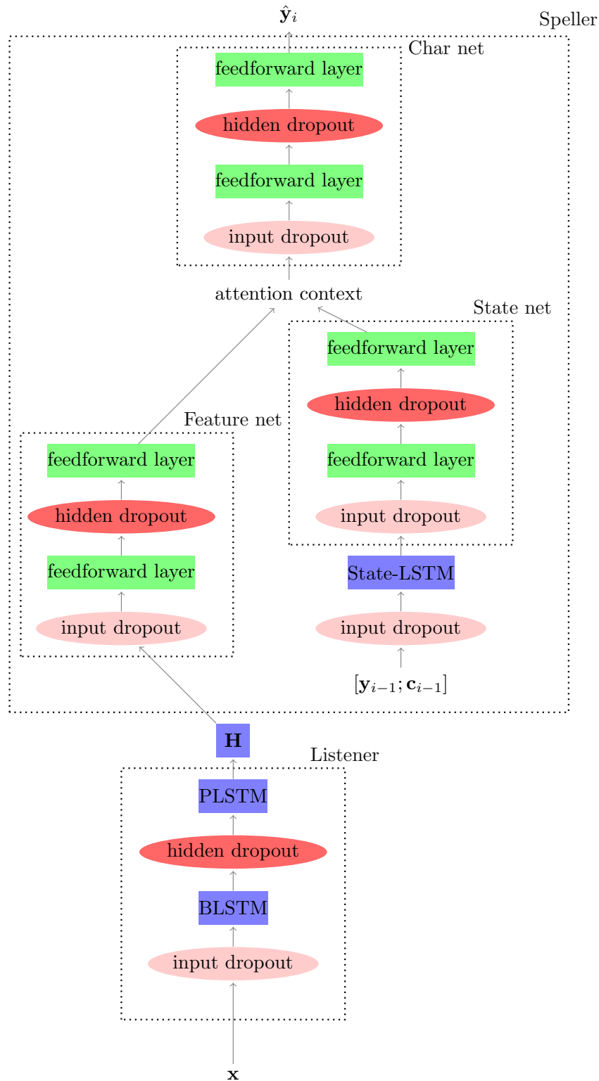
Figure 5.13: Listen attend and spell forward connections with added dropout. No recurrences are shown.
